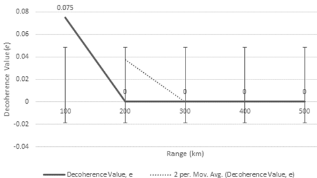
Figure 11. Decoherence vs Range plot for quantum radar.
