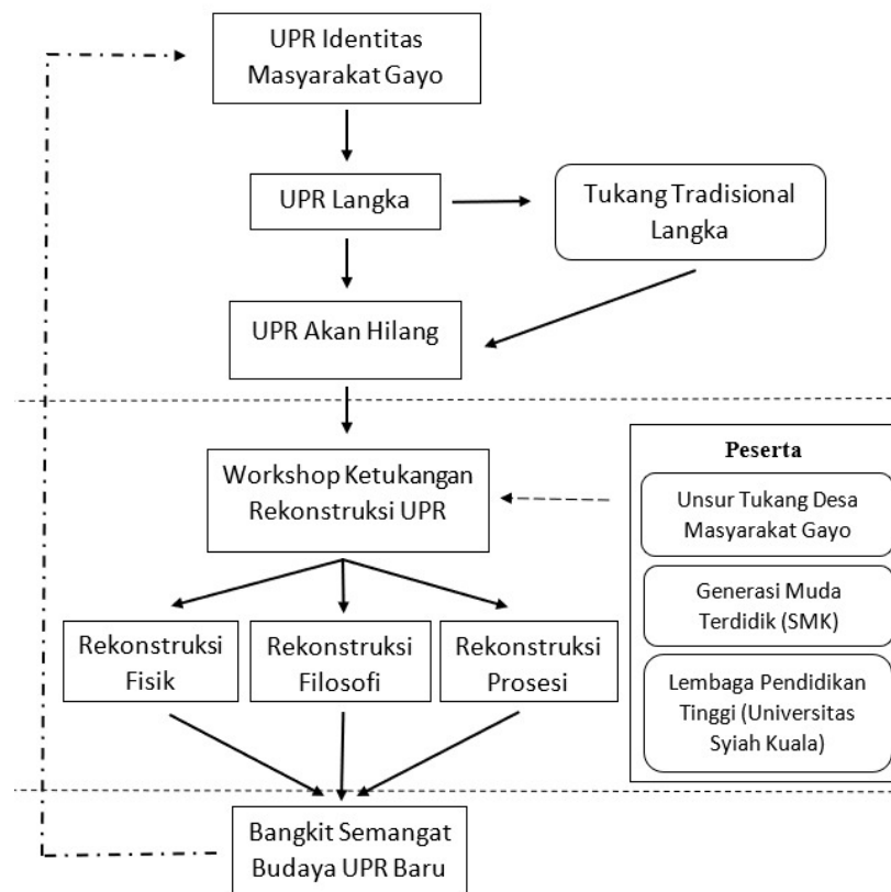
Gambar 2. Conceptual Framework
