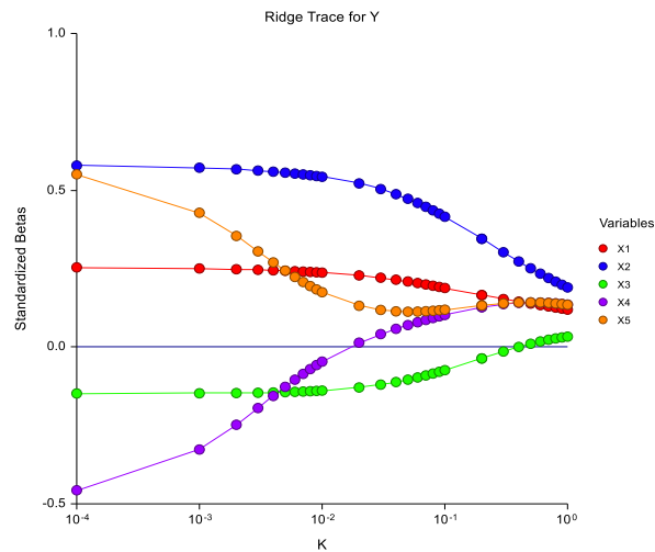
Gambar 1. Ridge Trace
