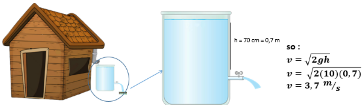
Figure 3. Tank's rainwater.
