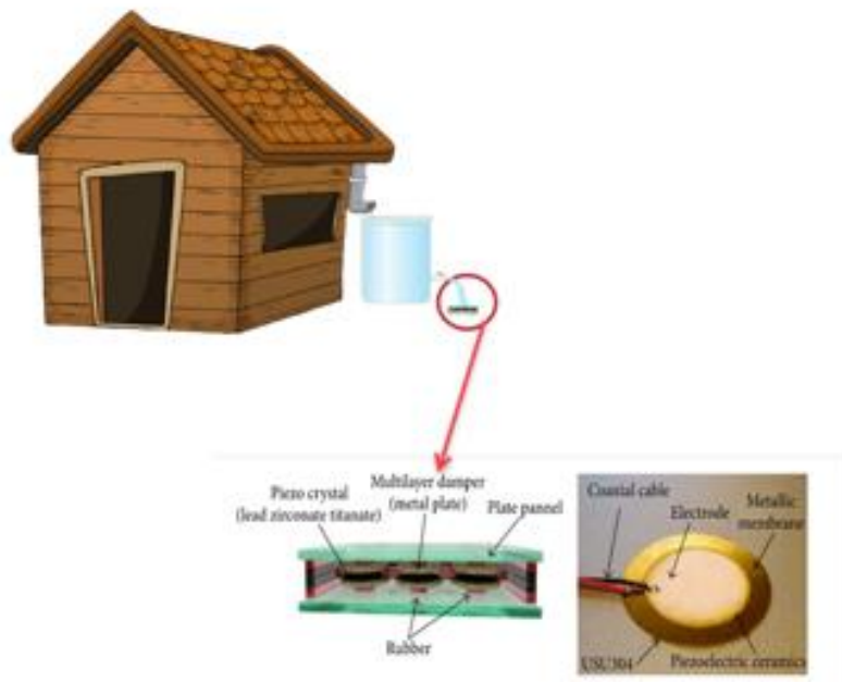
Figure 2. Model of rain water power plant using piezoelectric.
